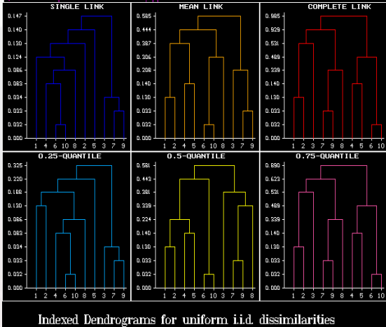
Indexed Dendrograms for uniform i.i.d. dissimilarities
